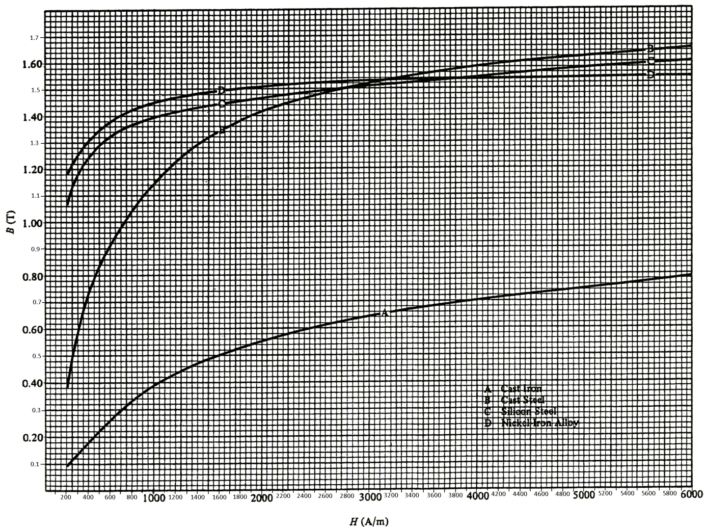
Fig. 11-13. B - H curves, H > 400 A/m
