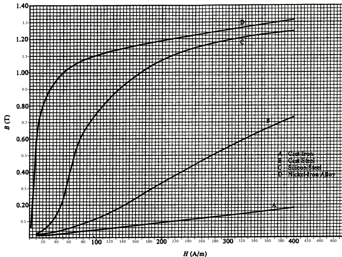
Fig. 11-12. B - H curves, H < 400 A/m
